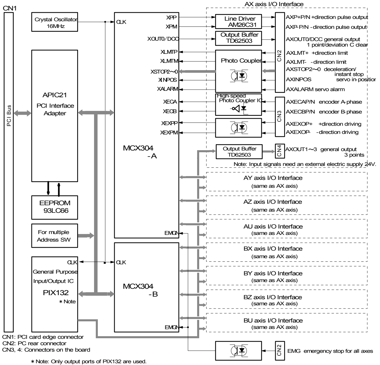
MC8082P Circuit Block Diagram
