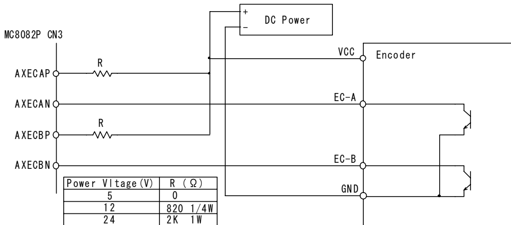
Connection Example with Open Collector Output
