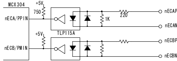
Encoder A/B phase Input Signal Circuit
